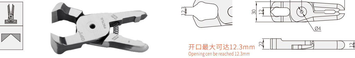
塑胶水口顶切平嘴钳 Plastic water top cutting flat nose pliers
