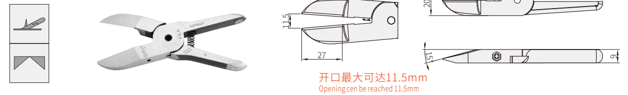
塑胶水口圆头斜嘴钳 Plastic water mouth round nose diagonal pliers
