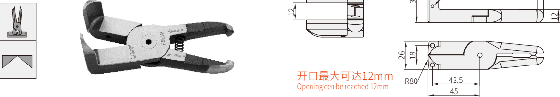
塑胶水口L形直角钳 Plastic spout L-shaped right Angle pliers
