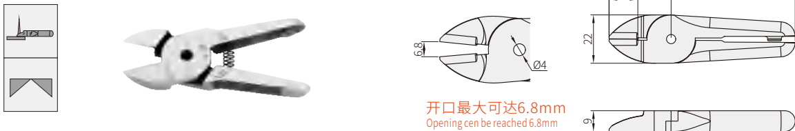
塑胶水口圆头平嘴钳 Straight blade
